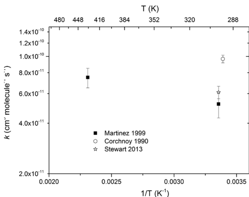
Rate coefficients for \text{NO}_3 + \text{terpinolene}
